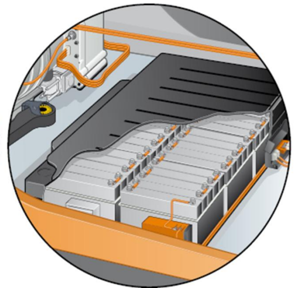
Harnessing for battery systems
