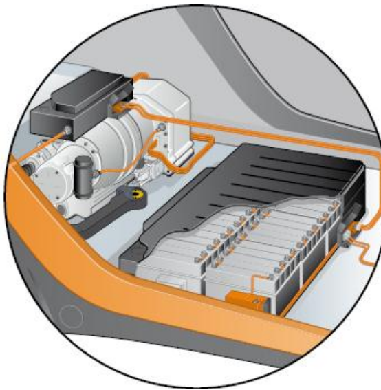
Drive system high-voltage harnessing
